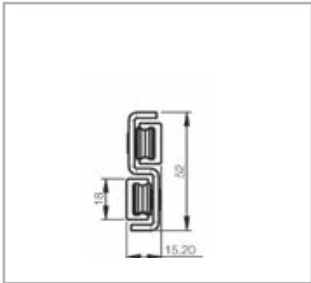
TLRD18 - TLRS18 Load capacity p. TLR-44
