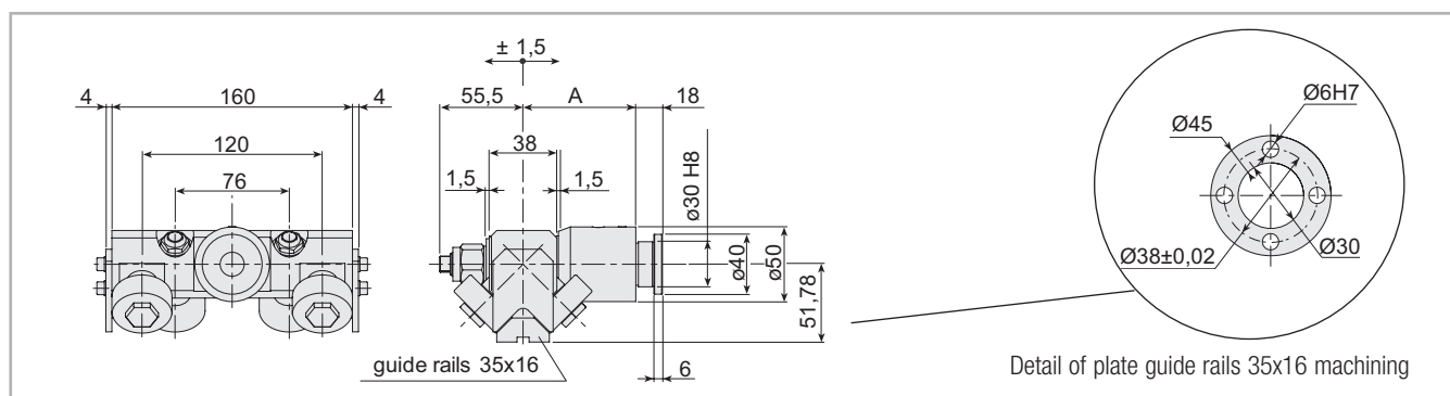
Important: remove the spacer washers to enable self-alignment of the roller slide
