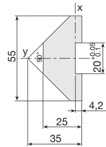
V-shaped guide rail 55x25
